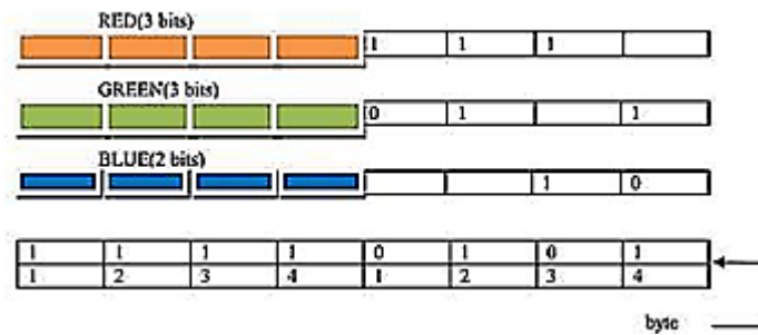
Figure 2. Hash-LSB Process
